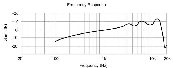
AT8139S Windscreen
