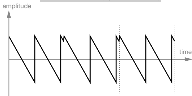
Main oscillator (synchronized)
