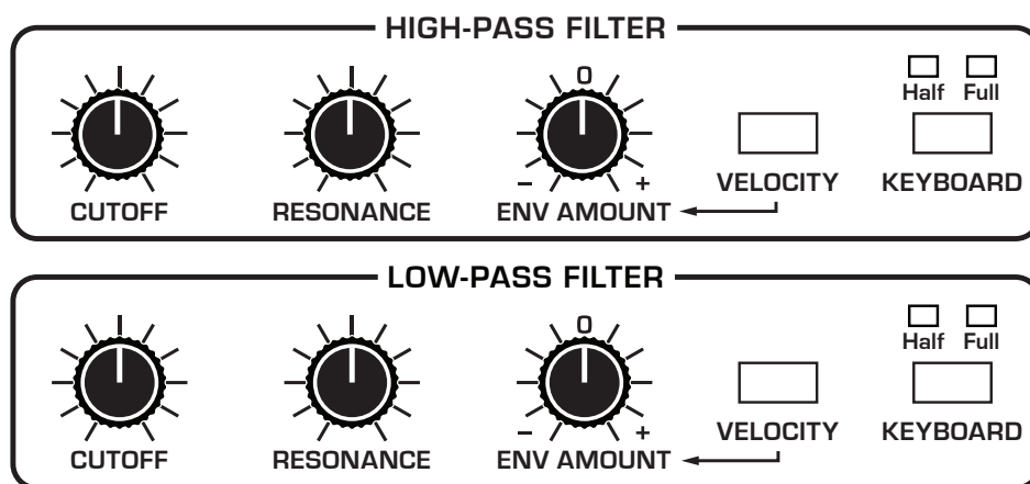
The Low-Pass Filter and High-Pass Filter
