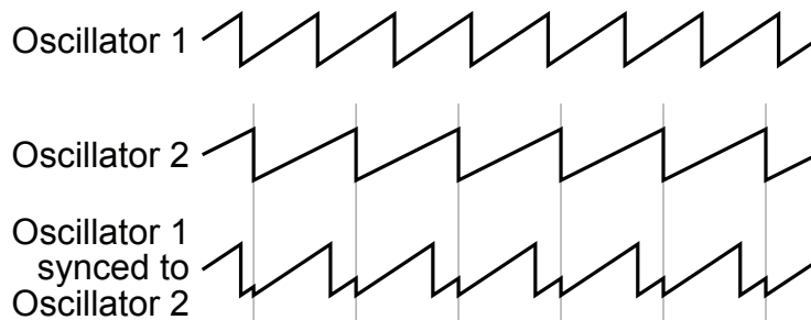
Oscillator hard sync
