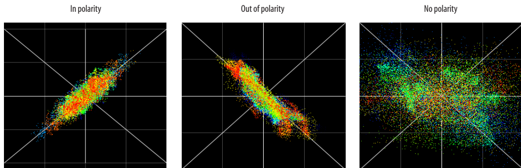
Figure 9-18: Checking polarity in a stereo signal with the X-Y Plot.
