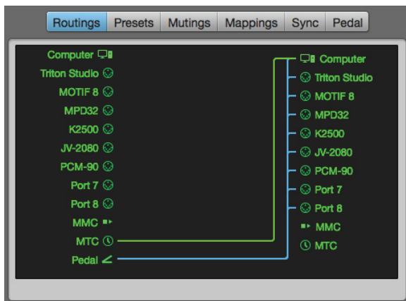
Figure 7-1: The connection from the MTC out port to the computer in port deliverers MIDI Time Code from the Express interface to software running on the computer.
