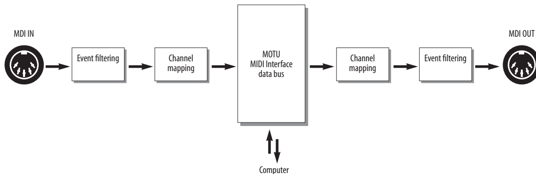
Figure 4-3: The path that MIDI data takes through a MOTU Express XT or micro express. Other MOTU interfaces do not provide MIDI processing.
