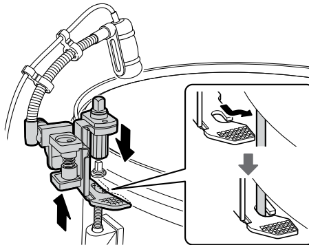
Drum mount's spring-loaded mechanism fastens it tightly to the drum rim/tension rod.
