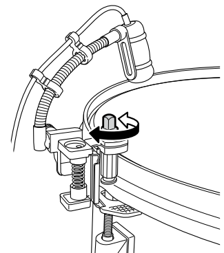
Mount design retains tuning key access to the tension rod.
