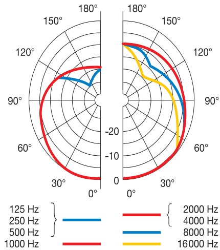
Diagrama polar C214
