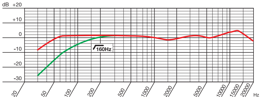
Frequenzgang C214
